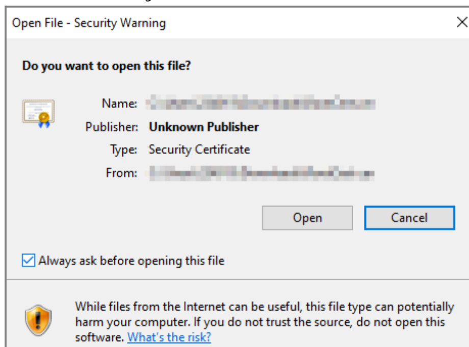
Figure 3-39 File download
