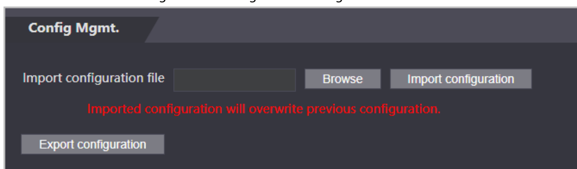
Figure 3-47 Configuration management
