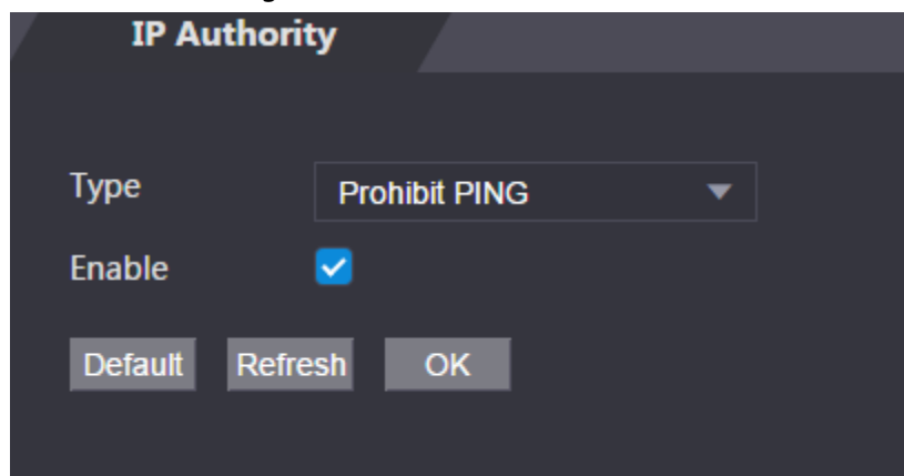
Figure 3-36 Prohibit PING
