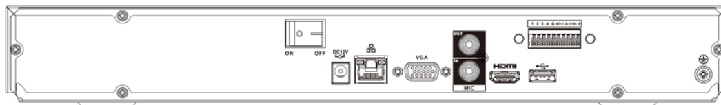
Figura 2-47 Panel trasero
