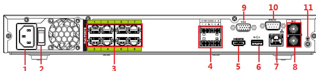
Figura 2-72 Panel trasero
