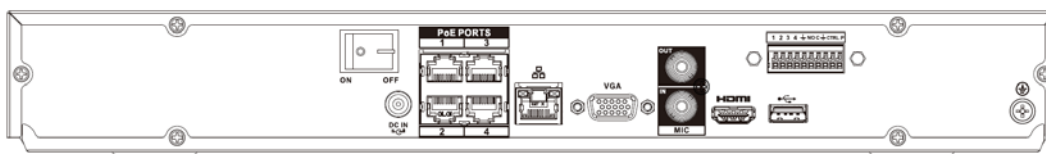
Figura 2-48 Panel trasero
