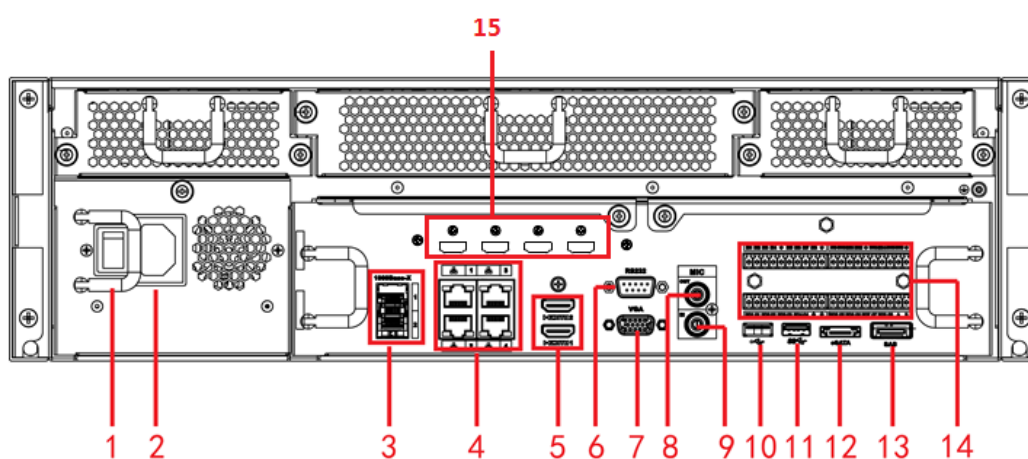
Figura 2-77 Panel trasero
