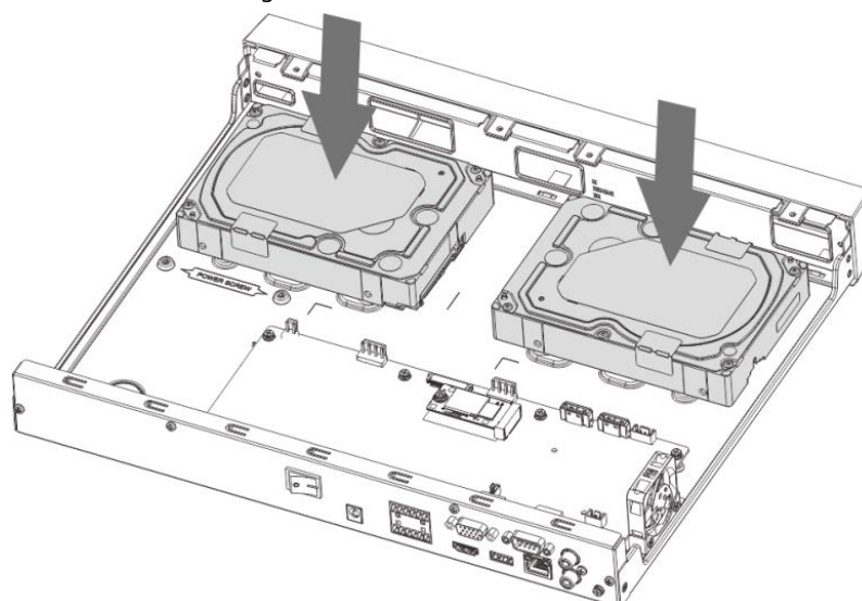
Figura 3-14 Alinear HDD
