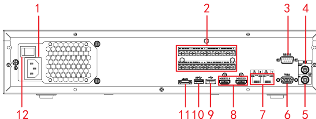
Figura 2-74 Panel trasero
