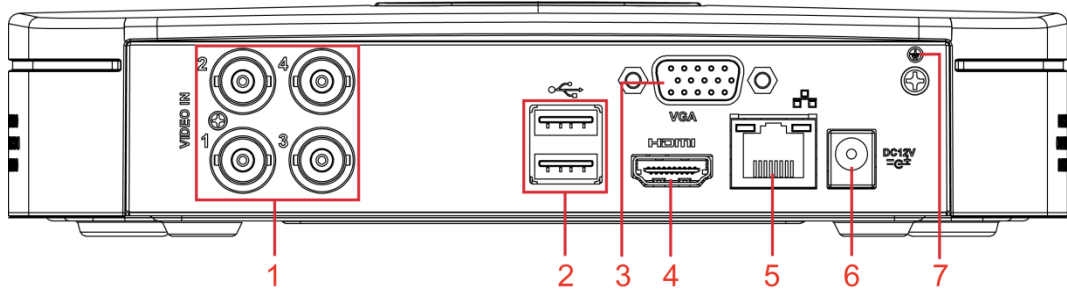
Figure 3-20 Panel trasero
