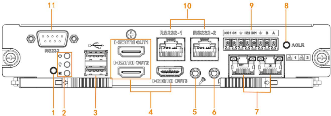
Figure 2-10 Master control board
