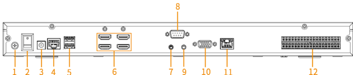
Figure 2-1 Rear panel
