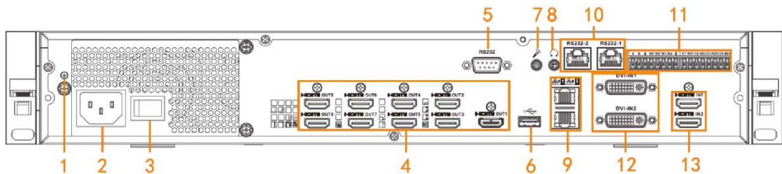
Figure 2-5 Rear panel
