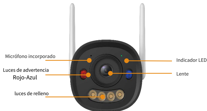
Vista frontal
