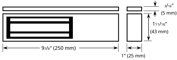
Electroimán
