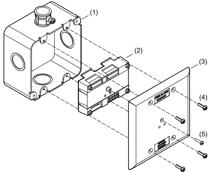
Figure 1: Installation diagram
