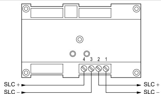
Figure 2: Wiring diagram
