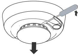
Figure 10.2: Remove the detector cap
