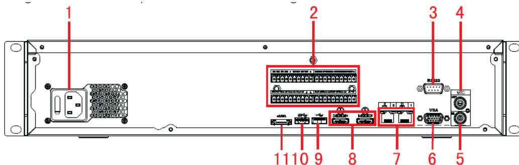
Figura 2-75 Panel trasero
