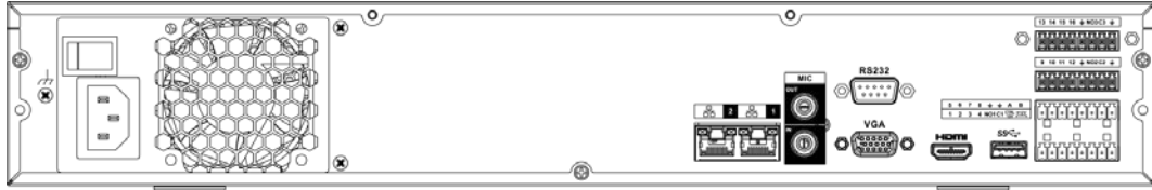
Figura 2-51 Panel trasero
