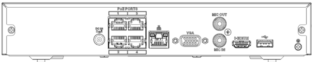
Figura 2-29 Panel trasero
