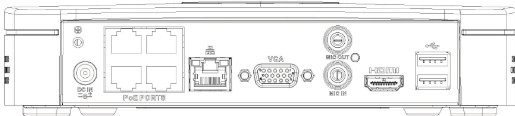
Figura 2-26 Panel trasero
