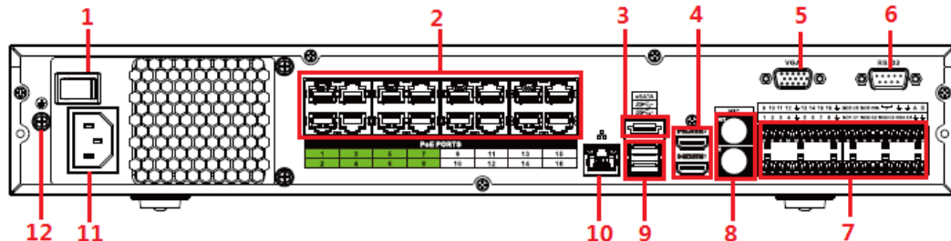
Figura 2-70 Panel trasero
