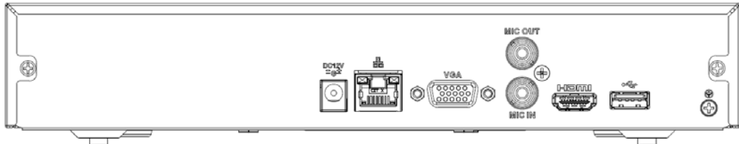
Figura 2-28 Panel trasero
