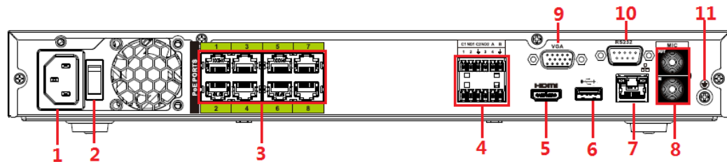
Figura 2-72 Panel trasero
