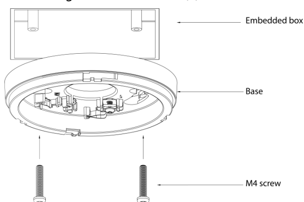
Figure 3-1 Installation (1)
