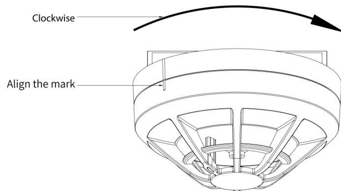
Figure 3-6 Installation (4)
