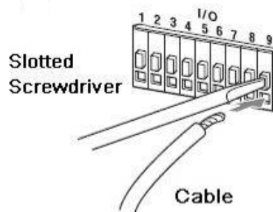
Figure 8-4 Install cable
