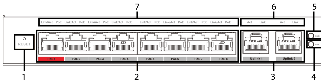
Figura 2-2 Panel frontal (16 puertos)
