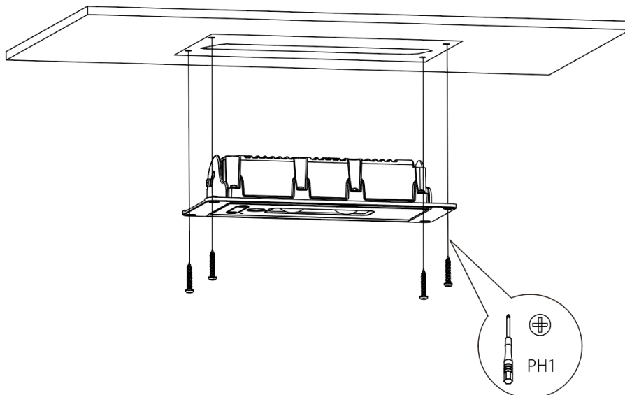
Figure 2-7 Fixing device (1)
