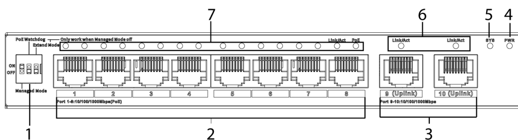
Figura 2-1 Panel frontal
