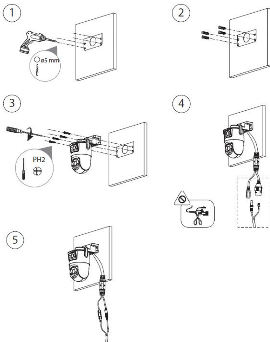
Figure 4-3 Wall mount
