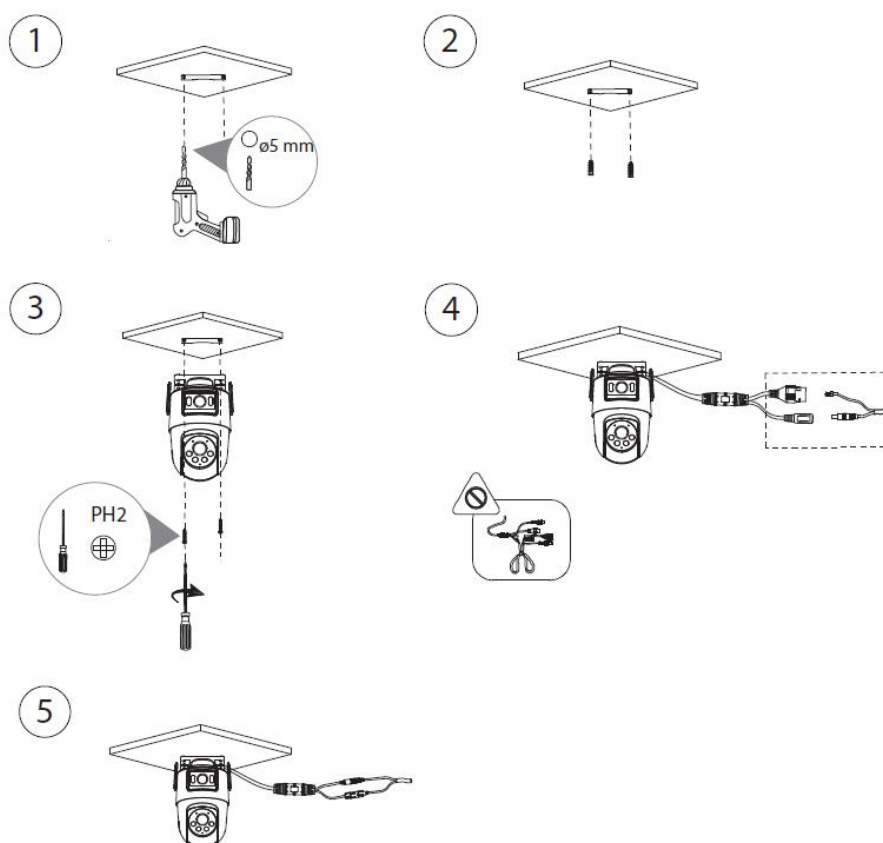
Figure 4-4 Ceiling mount
