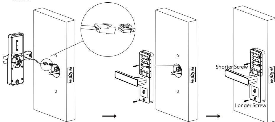
Interior Assembly Screws
