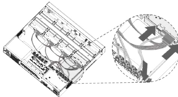
Figura 2-22 Conectar cables
