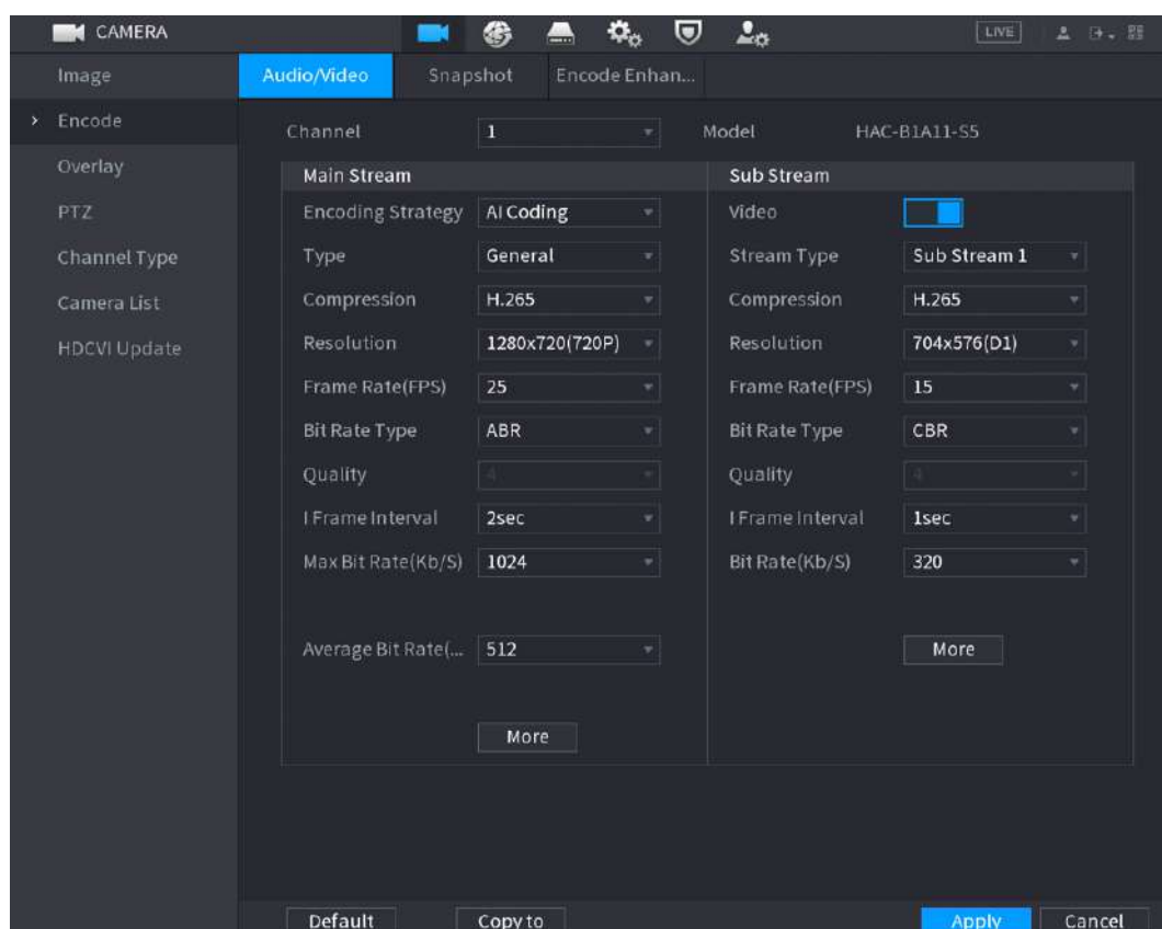
Figure 5-77 Audio/video
