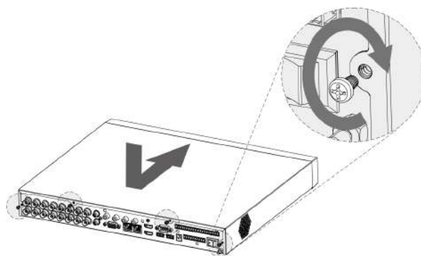
Figure 2-6 Put back cover
