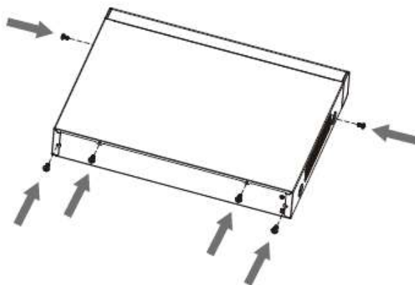
Figure 2-29 Fasten screws
