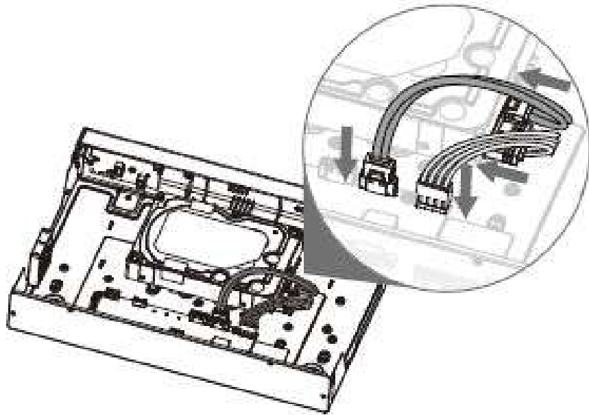
Figure 2-27 Connect cables
