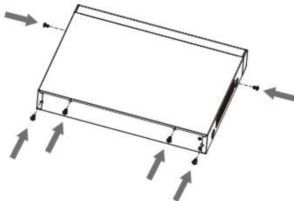
Figure 2-29 Fasten screws
