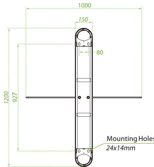
Bottom View
