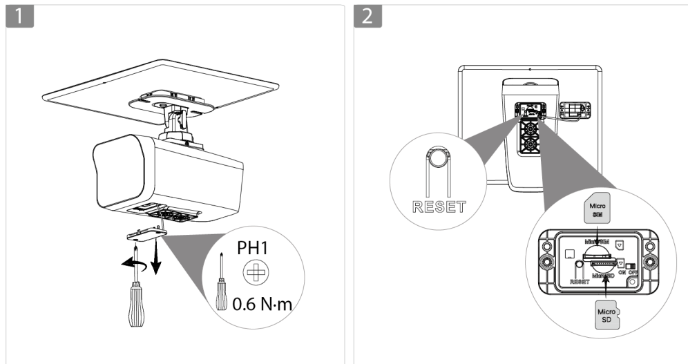
Figure 3-2 Install the SD/SIM card
