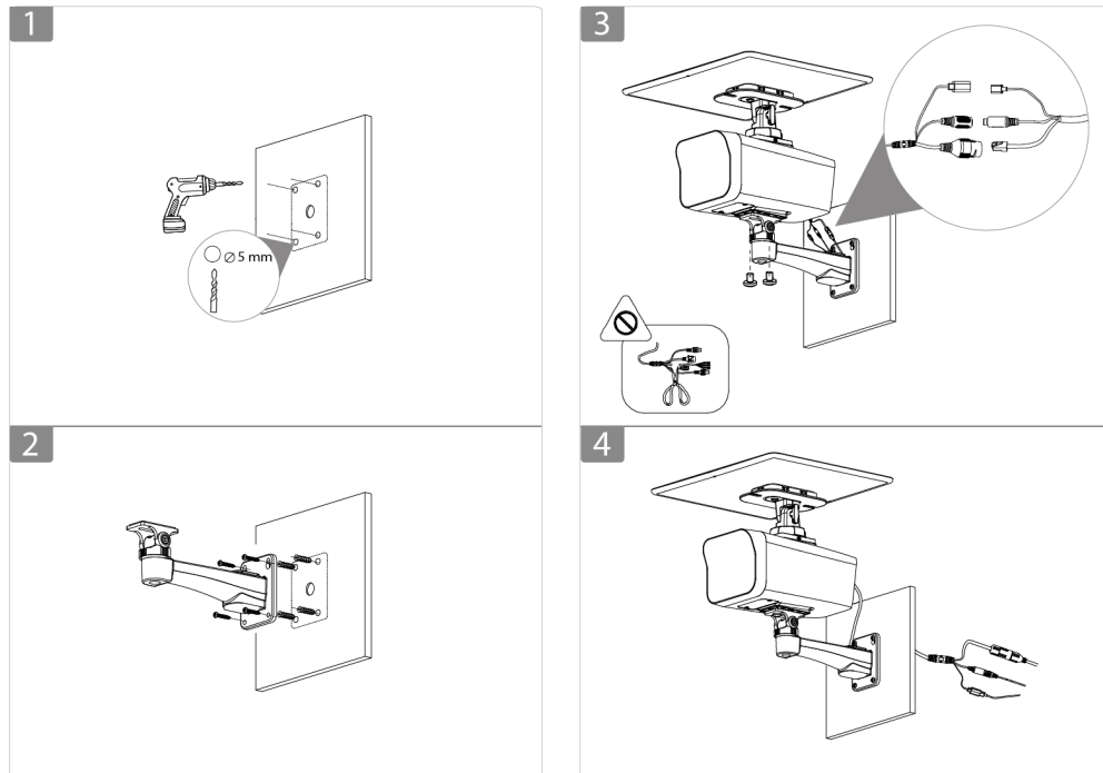
Figure 3-4 Cable going through the mounting surface
