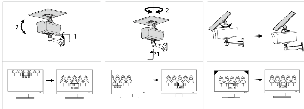
Figure 3-7 Adjust the lens angle
